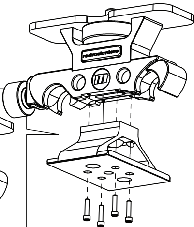
Required Screws
