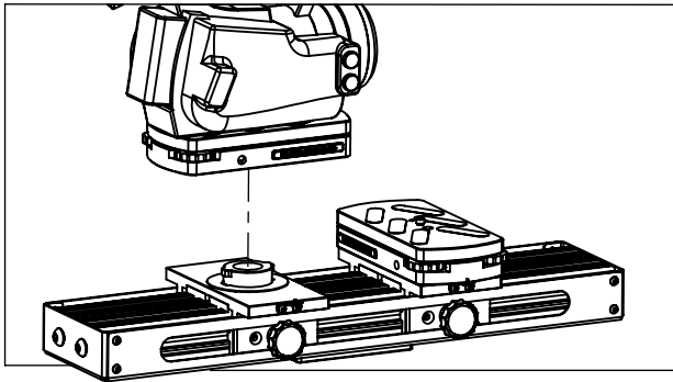
(3) Lower Camera / Camera Plate onto base. Rotate plate 90 degrees and tighten thumb screw to secure the camera. Repeat for second camera
