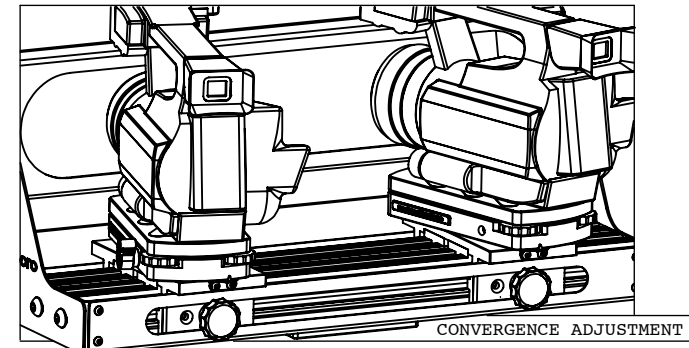
(5) Adjust Convergence by loosening thumb screw and rotating camera(s). You can use scale to adjust both cameras with precision and repeatability
