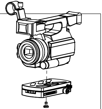
(2a) Remove Camera Plate from Interaxial Bar by turning the knob to loosen Plate, rotate 90 degrees and lift up
